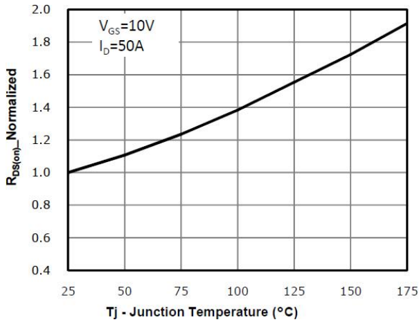
Figure 7. R_{ds(on)} -Junction Temperature( ^{\circ}\text{C} )
